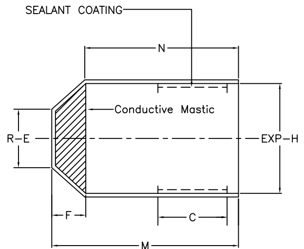
EXPANDED CONDUCTIVE END CAP
